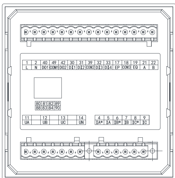
Figure 15 APM520 Extended Ethernet/Temperature, 10 - Measurement/Leakage Wiring Diagram
