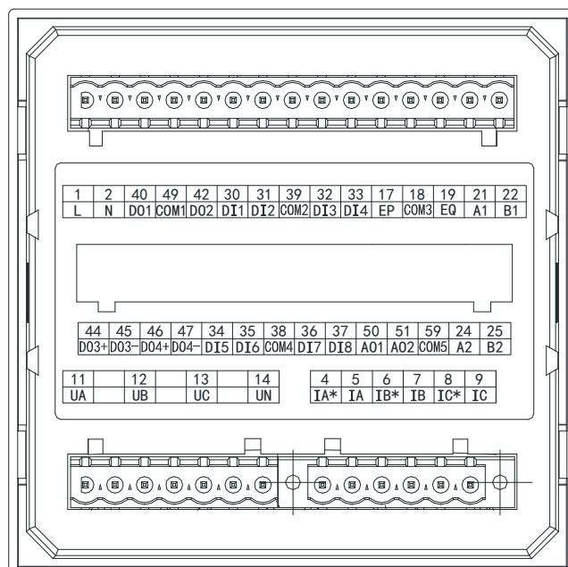
Figure 14 APM520 extended K/2M/2C wiring diagram
