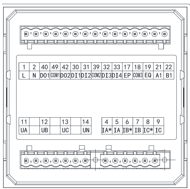
Figure 13 APM520 basic wiring diagram
