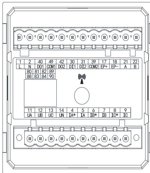
Figure 10 APM510 extended 4G/NB wiring diagram
