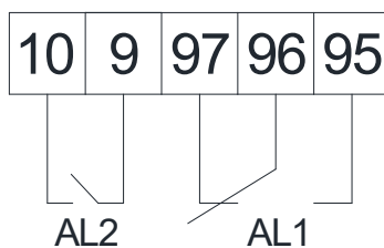
Relay output terminal (Dry Contact ) AL1: Alarm relay AL2: Warning relay
